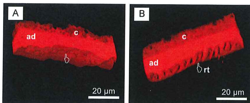
Fig. 8. CLSM 3D projections created following the specimen preparation and imaging procedures described by Sauro et al., [88] using Rhodamine-B to dope self-etching adhesives. A: CLSM projection image (fluorescence – Rhodamine B) of a self-etching adhesive applied on dentine air-abraded using Aquacut Quattro (VELOPEX International) with BAG 4555 (Sylc, OSSpray). Note the bottom part of the adhesive layer (ad) is characterised by an absence of resin tags (rt) or by one few very short (< 2 μm) resin tags (pointer) probably due to BAG-occluded dentine tubules. B: CLSM projection image (fluorescence – Rhodamine B) of a self-etching adhesive applied on smear-layer covered dentine. Note the bottom part of the adhesive layer (ad) contains numerous short (> 2 μm) resin tags (pointer) probably due to BAG-occluded dentine tubules. (All the images in this figure are original and never published before).
